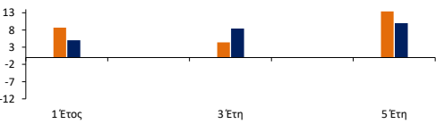
Cumulative Performance (%)
